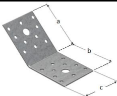
Uholník KLR - 135° zinok
